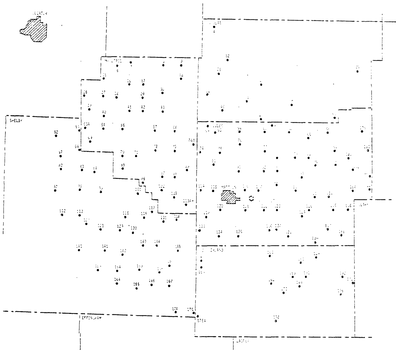
Figure 1. Raingauge network established for rainfall measurements during August 4-31, 1976
