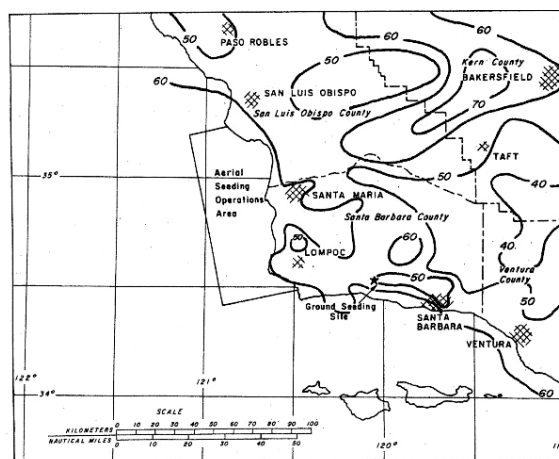
Fig. 7 Percentage of Winter Precipitation Associated with Convection Bands
