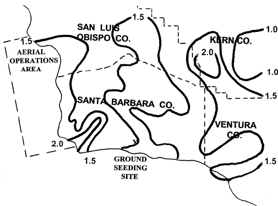
Fig. 5 Seed/no-seed Ratios, Phase II (aerial)
