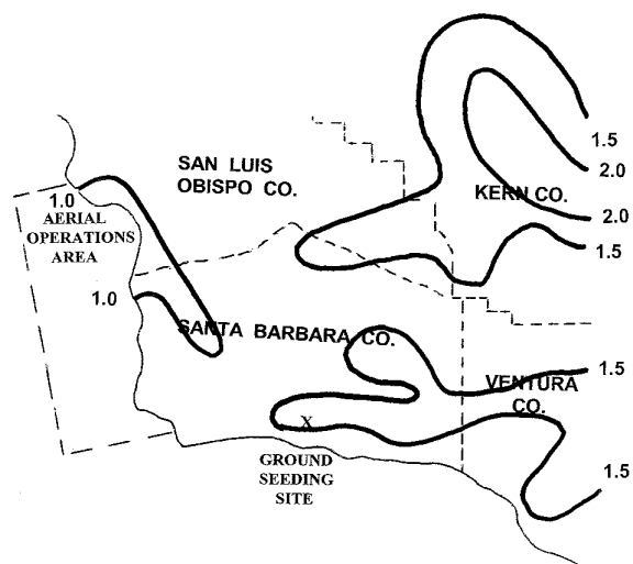
Fig. 3 Seed/no-seed Ratios, Phase I (ground)
