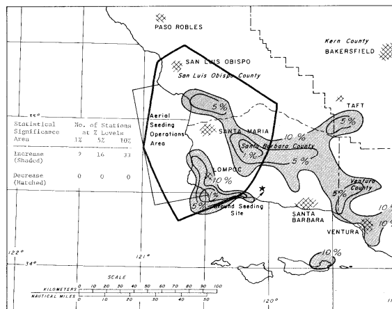
Fig. 6 Statistical Significance of Airborne Seeding
