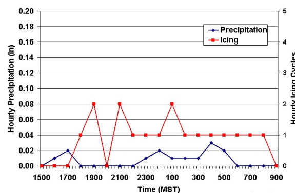
Figure 7. Hourly precipitation and riming rates, January 27-28, 2004
