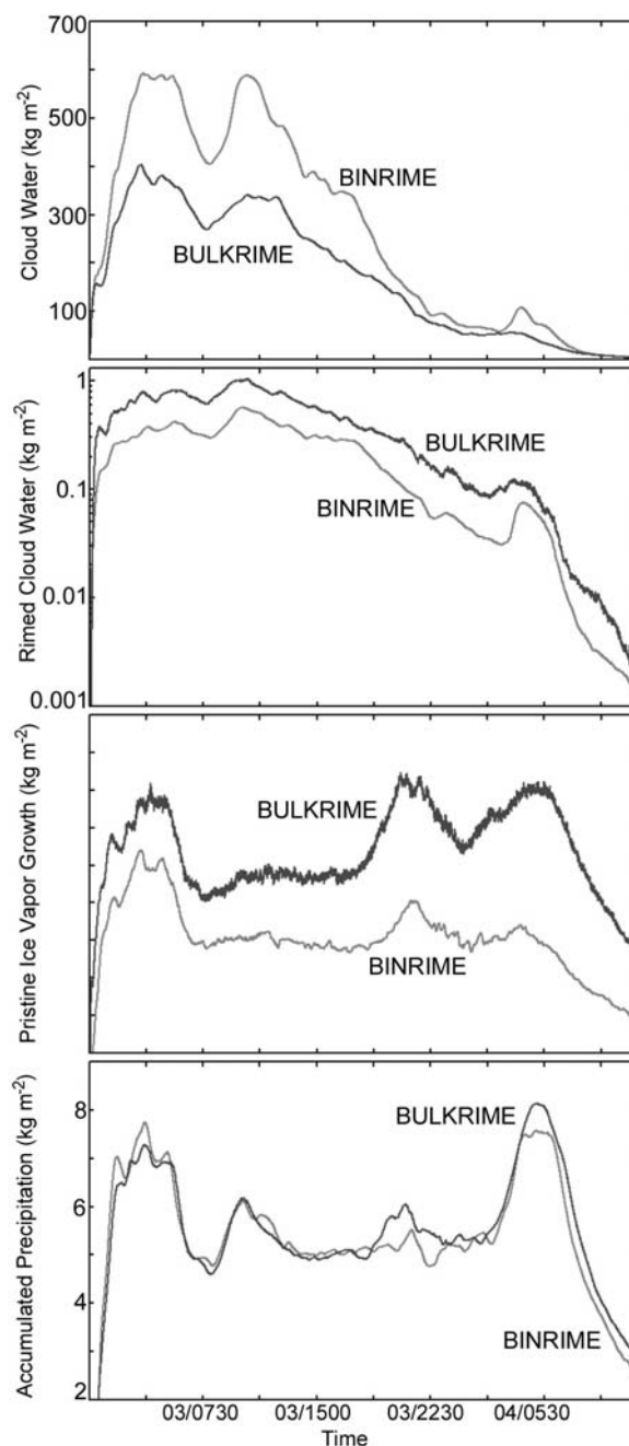
Figure 12. Time series of domain-summed quantities comparing use of the old fall speed power laws and bulk riming (BULK) with the new fall speed power laws and binned riming (BINRIME) in grid 3. Panel (a) displays cloud water, (b) amount of rime, (c) vapor growth of pristine ice, and (d) accumulation of precipitation. Units of ( \text{kg m}^{-2} ) denote vertically integrated quantities. Multiplying by area of the domain gives mass totals.
