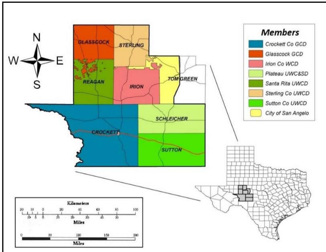
Figure 3: The West Texas Weather Modification Association target area
