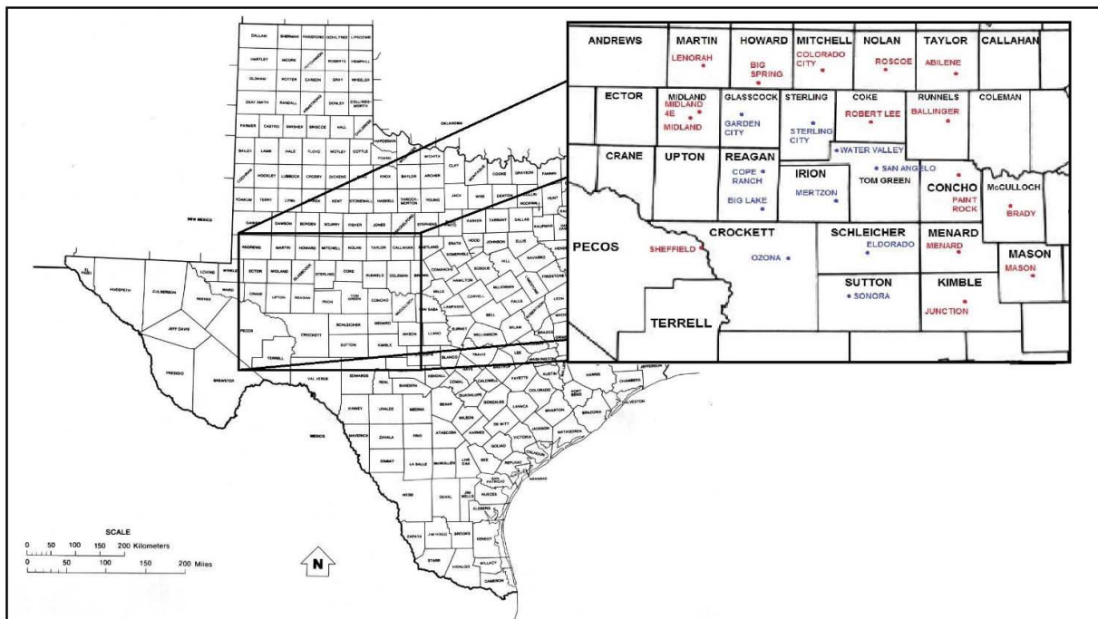
Figure 5: Rain Gauge Locations within (blue labels) and outside (red labels) of the target area.
