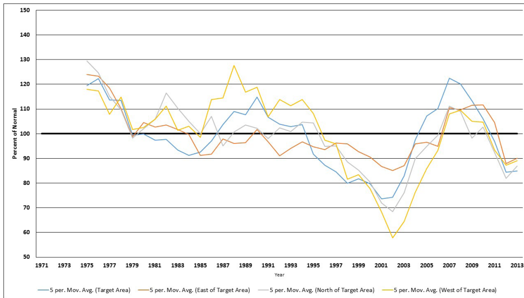
Figure 7: Percent relative to average rainfall within the target (blue line) area, east (orange line) of the target area, north (gray line) of the target area, and west (yellow line) of the target area.
