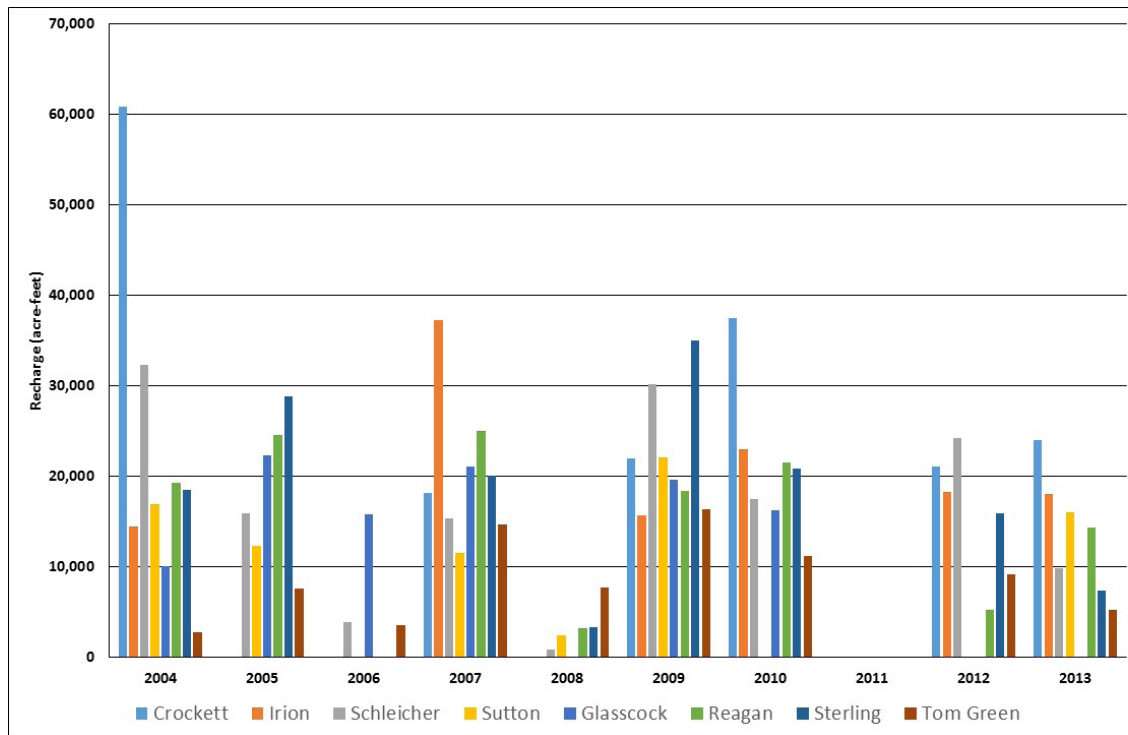
Figure 8: Estimated recharge for each county in the West Texas Weather Modification Association target area (2004–2013).
