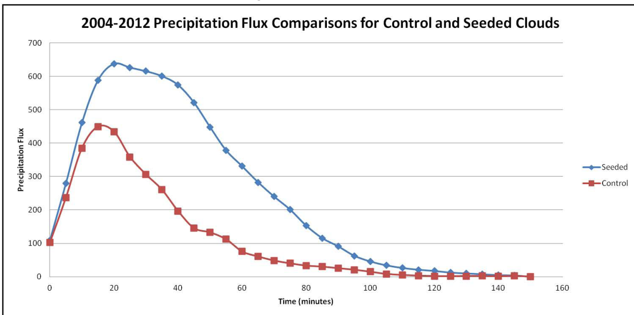
Figure 4: Precipitation flux (2004-2012) for seeded clouds versus control clouds (Ruiz-Columbi   et al., 2014). (kg/m 2 -s)
