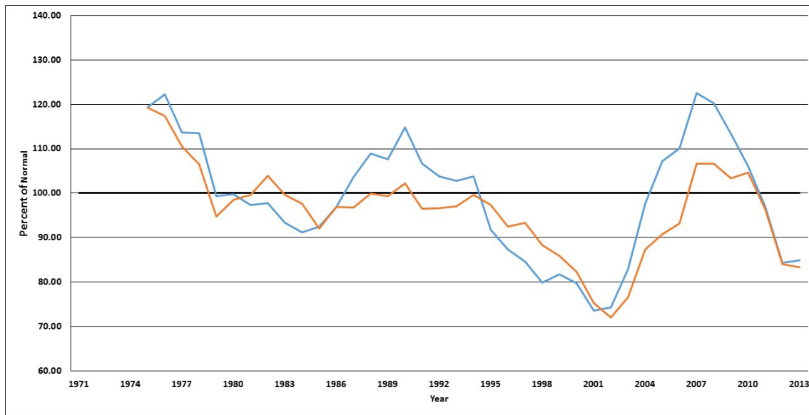
Figure 6. Percent relative to average rainfall relative to the period 1971–2013 within the West Texas Weather Modification Association target area (blue line) compared with outside (orange line) the target area.
